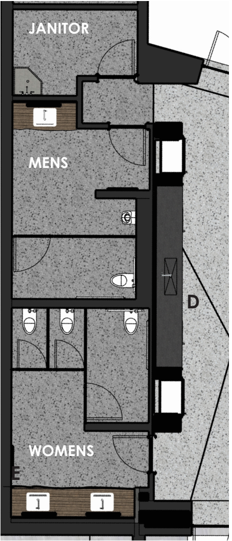
FLOOR PLAN 1/8"=1'-0"
