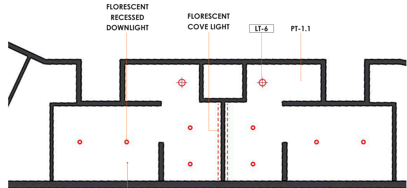
REFLECTIVE CEILING PLAN 1/4"=1'-0"
