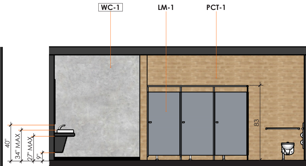
B2 - SECTION ELEVATION 3/16"=1'-0"
