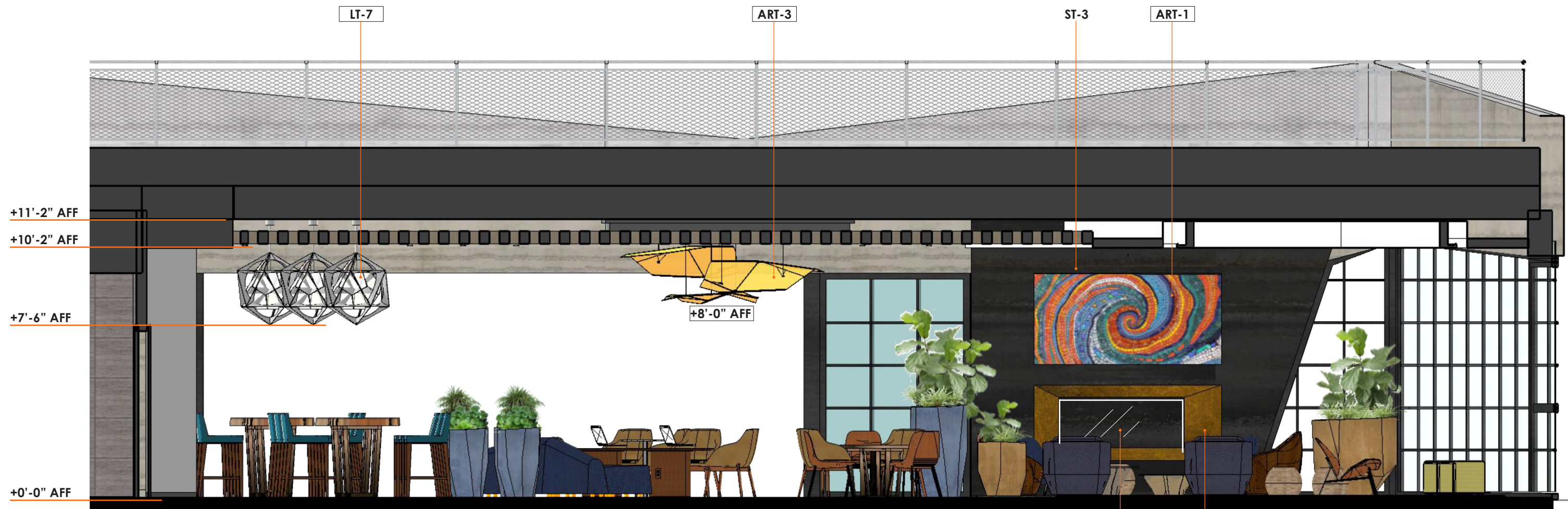
SECTION ELEVATION 1/4"=1'-0"
